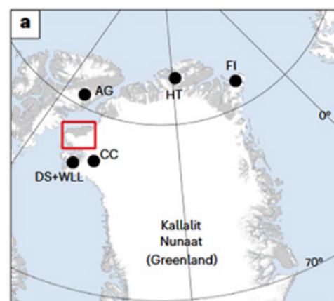
Fig. 1 | Maps of study area. a , Map of Greenland and surrounding areas with modern ice extents 27 showing study site in red box and the locations of Hans Tausen (HT) and Flade Isblink (FI) ice caps, the Camp Century ice core site (CC), the Agassiz Ice Cap ice core site (AG) and Deltasø (DS) and Wax Lips (WLL) lakes.
