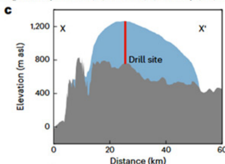
c , Cross section shows ice thickness and bedrock topography of Prudhoe Dome
