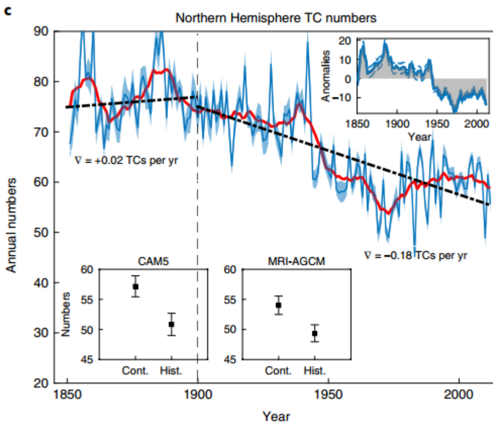
Bild 15 (Teilbild) [15] Fig. 1 Anthropogenic greenhouse warming-induced changes in global and hemispheric annual TC numbers as inferred from the 20CR dataset and changes in the mean annual TC numbers between the pre-industrial
