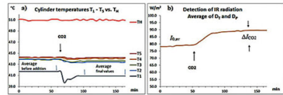
Fig. 17: Effects of 8% CO 2 . a) Decrease in cylinder temperatures, b) increase in IR radiation after adding CO 2 (WV concentration about 0.15%).
