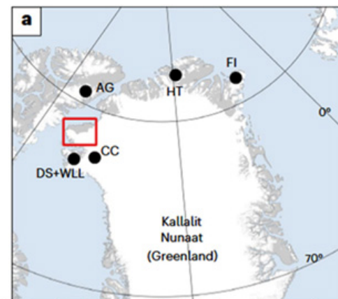
Fig. 1 | Maps of study area. a, Map of Greenland and surrounding areas with modern ice extents 21 showing study site in red box and the locations of Hans Tausen (HT) and Flade Isblink (FI) ice caps, the Camp Century ice core site (CC), the Agassiz Ice Cap ice core site (AG) and Deltasø (DS) and Wax Lips (WLL) lakes.
