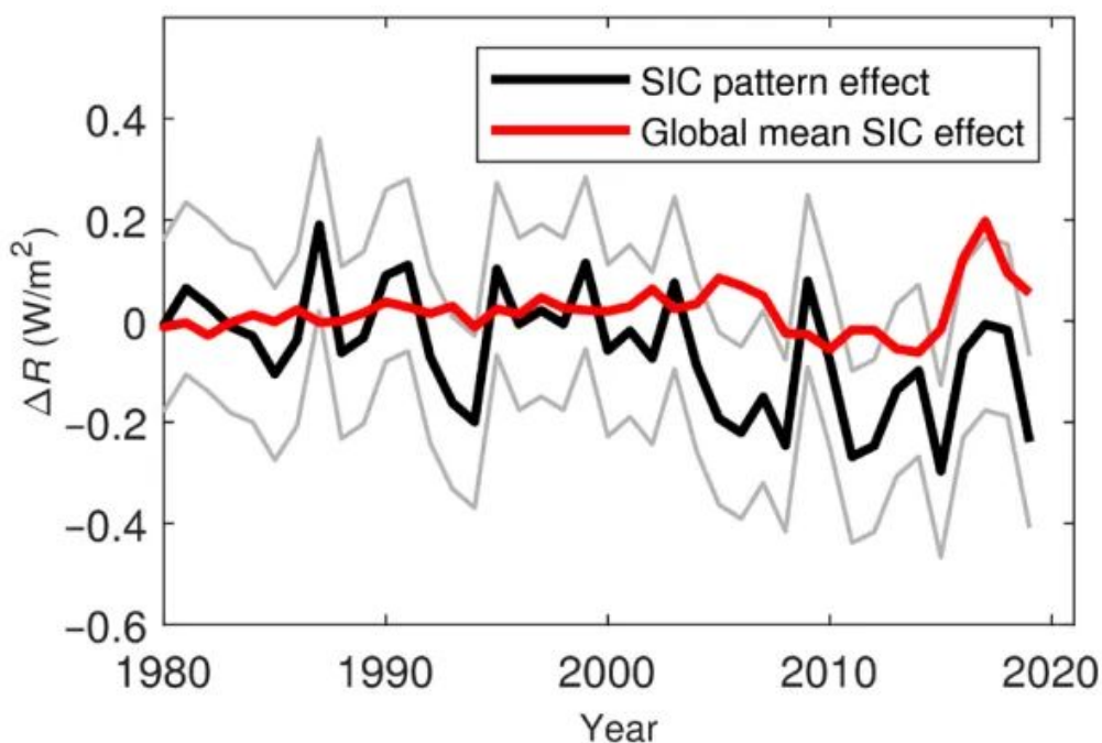
Fig. 3. Decomposition of SIC-induced radiation anomalies at TOA. The red line is the radiative effect of global mean SIC anomalies ( \lambda_{\text{SIC}}\Delta\text{SIC} ), and the black line is the SIC pattern effect ( P_{\text{SIC}} ; see Eq. 7 in Materials and Methods). The gray lines denote the SD interval of the SIC pattern effect.
