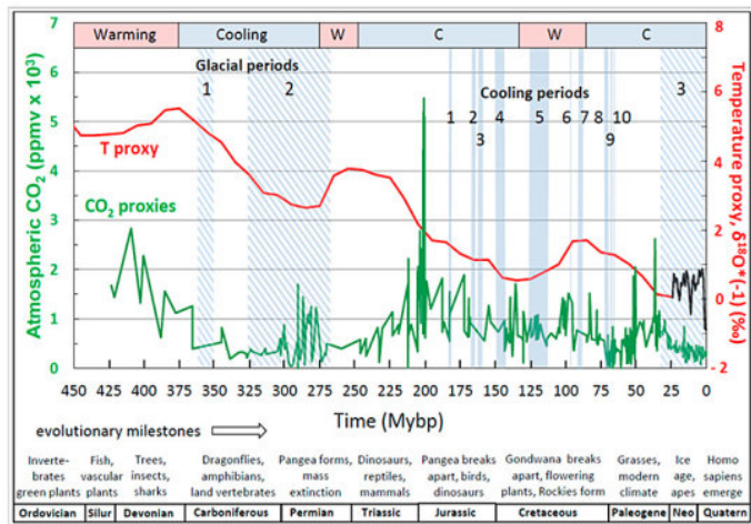
Figure 5. Temperature (T) and atmospheric carbon dioxide (CO 2 ) concentration proxies during the Phanerozoic Eon. Time series of the global temperature proxy ( \delta^{18}O_{T-1} , red curve, n = 6689 ) are from Prokoph et al. [26] while concurrent atmospheric CO 2 concentration proxies (green curve, n = 831 ) are from Royer [40]. The red curve plots moving averages of the non-detrended T proxy averaged in 50 Myr windows incremented in ten-Myr steps (the 10–50 Myr moving average in Figure 3b). The green curve shows mean CO 2 concentration values in one-Myr bins averaged over high-resolution portions of the CO 2 record (the most recent Phanerozoic) and linearly interpolated over low-resolution portions (the older Phanerozoic). Glaciations based on independent sedimentary evidence are designated by vertical blue cross-hatched areas, while putative cool periods are designated by vertical solid blue bars. Major cooling and warming cycles are shown by the colored bars across the top while geological periods and evolutionary milestones are shown across the bottom. Abbreviations: CO 2 , atmospheric concentration of carbon dioxide based on various proxies (Methods); ppmv, parts per million by volume; Silu., Silurian; Neo, Neogene; Quatern., Quaternary. The three major glacial periods and ten cooling periods identified by blue cross-hatches and solid lines, respectively, are (after [21]): Glacial periods. 1. late Devonian/early Carboniferous; 2. Permian-Carboniferous; 3. late Cenozoic. Cooling periods. 1. late Devonian/early Carboniferous; 2. Bathonian; 3. late Carboniferous to mid-Ordovician; 4. Tithonian to early Permian; 5. Apelian; 6. mid-Cenomanian; 7. mid-Turonian; 8. Campanian-Maastrichtian boundary; 9. mid-Maastrichtian; 10. late-Maastrichtian.
