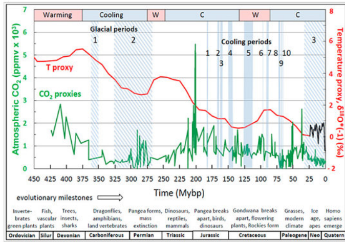
Figure 5. Temperature (T) and atmospheric carbon dioxide (CO 2 ) concentration proxies during the Phanerozoic Eon. Time series of the global temperature proxy ( \delta^{18}O_1 -1), red curve, n = 6800 ) are from Prokoph et al. [28] while concurrent atmospheric CO 2 concentration proxies (green curve, n = 831 ) are from Royer [40]. The red curve plots moving averages of the non-detrended T proxy averaged in 50 My windows incremented in ten-My steps (the 10-50 My moving average in Figure 3b). The green curve shows mean CO 2 concentration values in one-My bins averaged over high-resolution portions of the CO 2 record (the most recent Phanerozoic) and linearly interpolated over low-resolution portions (the older Phanerozoic). Glaciations based on independent sedimentary evidence are designated by vertical blue cross-hatched areas, while putative cool periods are designated by vertical solid blue bars. Major cooling and warming cycles are shown by the colored bars across the top while geological periods and evolutionary milestones are shown across the bottom. Abbreviations: CO 2 , atmospheric concentration of carbon dioxide based on various proxies (Methods); ppmv, parts per million by volume; Silu., Silurian; Neo, Neogene; Quatern, Quaternary. The three major glacial periods and ten cooling periods identified by blue cross-hatches and solid lines, respectively, are (after [21]): Glacial periods. 1. late Devonian/early Carboniferous; 2. Permian-Carboniferous; 3. late Cenozoic. Cooling periods. 1. late Devonian/early Carboniferous; 2. Bathonian; 3. late Carboniferous to mid-Ordovician; 4. Tithonian to early Permian; 5. Aptian; 6. mid-Cenomanian; 7. mid-Turonian; 8. Campanian-Maastrichtian boundary; 9. mid-Maastrichtian; 10. late-Maastrichtian.
