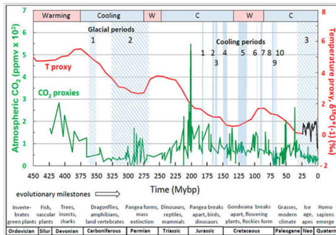
Figure 5. Temperature (T) and atmospheric carbon dioxide (CO 2 ) concentration proxies during the Phanerozoic Eon. Time series of the global temperature proxy ( \delta^{18}O_{T-1} ), red curve, n = 6889 ) are from Prokoph et al. [26] while concurrent atmospheric CO 2 concentration proxies (green curve, n = 831 ) are from Royer [40]. The red curve plots moving averages of the non-detrended T proxy averaged in 50 Myr windows incremented in ten-Myr steps (the 10–50 Myr moving average in Figure 3b). The green curve shows mean CO 2 concentration values in one-Myr bins averaged over high-resolution portions of the CO 2 record (the most recent Phanerozoic) and linearly interpolated over low-resolution portions (the older Phanerozoic). Glaciations based on independent sedimentary evidence are designated by vertical blue cross-hatched areas, while putative cool periods are designated by vertical solid blue bars. Major cooling and warming cycles are shown by the colored bars across the top while geological periods and evolutionary milestones are shown across the bottom. Abbreviations: CO 2 , atmospheric concentration of carbon dioxide based on various proxies (Methods); ppmv, parts per million by volume; Silu., Silurian; Neo., Neogene; Quatern., Quaternary. The three major glacial periods and ten cooling periods identified by blue cross-hatches and solid lines, respectively, are (after [21]): Glacial periods. 1. late Devonian/early Carboniferous; 2. Permian-Carboniferous; 3. late Cenozoic. Cooling periods. 1. late Devonian/early Carboniferous; 2. Bathonian; 3. late Carboniferous to mid-Ordovician; 4. Tithonian to early Permian; 5. Apelian; 6. mid-Cenomanian; 7. mid-Turonian; 8. Campanian-Maastrichtian boundary; 9. mid-Maastrichtian; 10. late-Maastrichtian.
