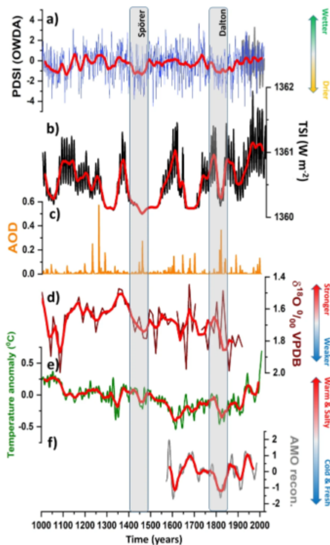
Fig. 5: Climate variability over the last millennium.
