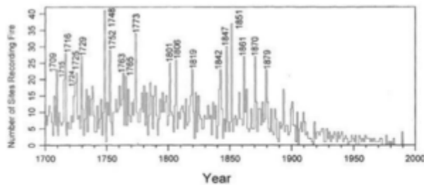
Bild 1 [3] Figure from Swetnam (1999) Historical Fire Regime Patterns in the Southwestern United States...
