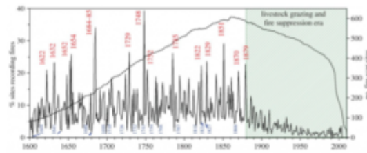
(c) A smaller and more precise record: fires in Yosemite National Park. Peaked in mid-19th C. "Climatic and human influences on fire regimes in mixed conifer forests in Yosemite National Park, USA" by Alan H. Taylor and Andrew E. Scholl in Forest Ecology and Management , 1 March 2012 (gated). Different data, same pattern -- a peak in the mid-19th century, followed by a long decline. Click to enlarge.
