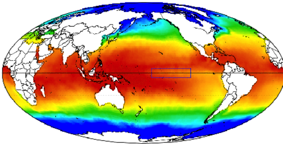
Monthly Sea Surface Temperature, Nov 1981 - Dec 2018 Reynolds Optimally Interpolated Dataset
