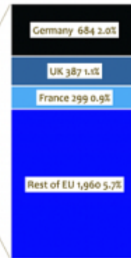
Global CO2 emissions 2019: '000,000 tonnes - percentages BPDData total 2019 CO2 emissions: 34,169,000,000 tonnes
