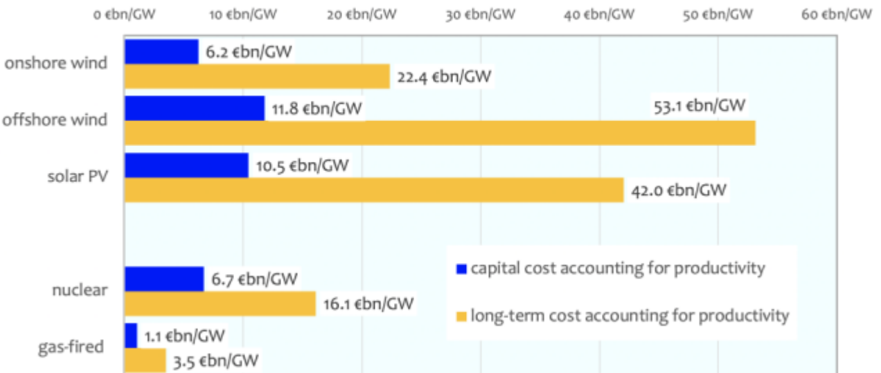
EU(28) Capital and Long-term cost of Generation technologies compared
