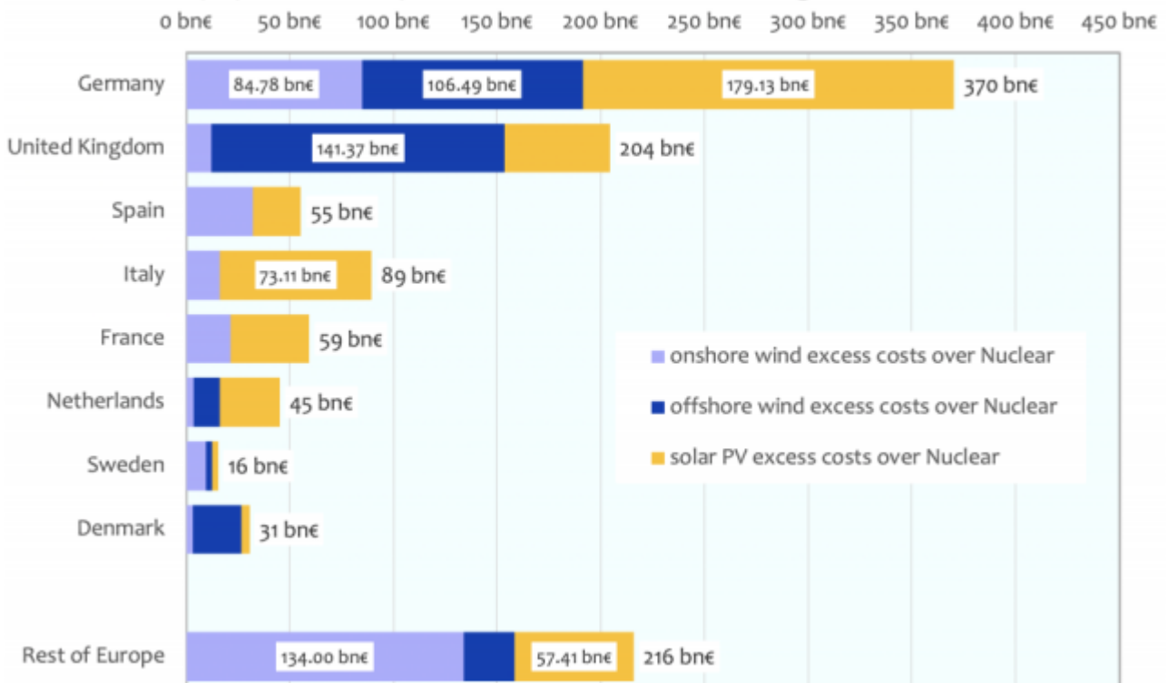
EU(28) Weather Dependent Renewables excess long-term costs: 2020
