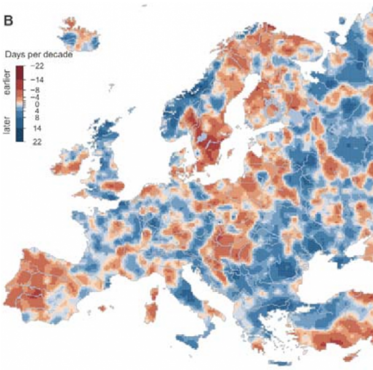
Bild 14 [x] Supplement, Fig. S3 (Teilbild) 7-day maximum precipitation (1960-2010), trend in timing; red indicates earlier precipitation, blue later precipitation (days per decade) (B).
