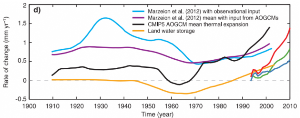
Bild 25 IPCC AR5 Figure 13.4 (Bilddauszug): (d) are matched to earlier panels. (Updated) from Church et al., 2013)
