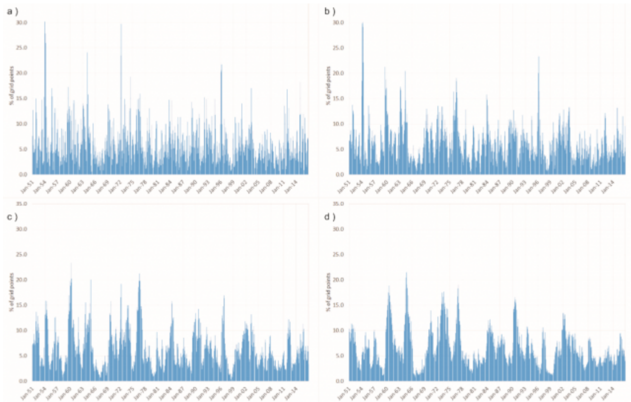
Figure 2. Temporal evolution of the percentage of grid points which fell within severe or extreme dry conditions (Standardized Precipitation Index SPI < -1.5 ) for the period 1951–2016. (a) 3-month SPI; (b) 6-month SPI; (c) 12-month SPI, and (d) 24-month SPI.
