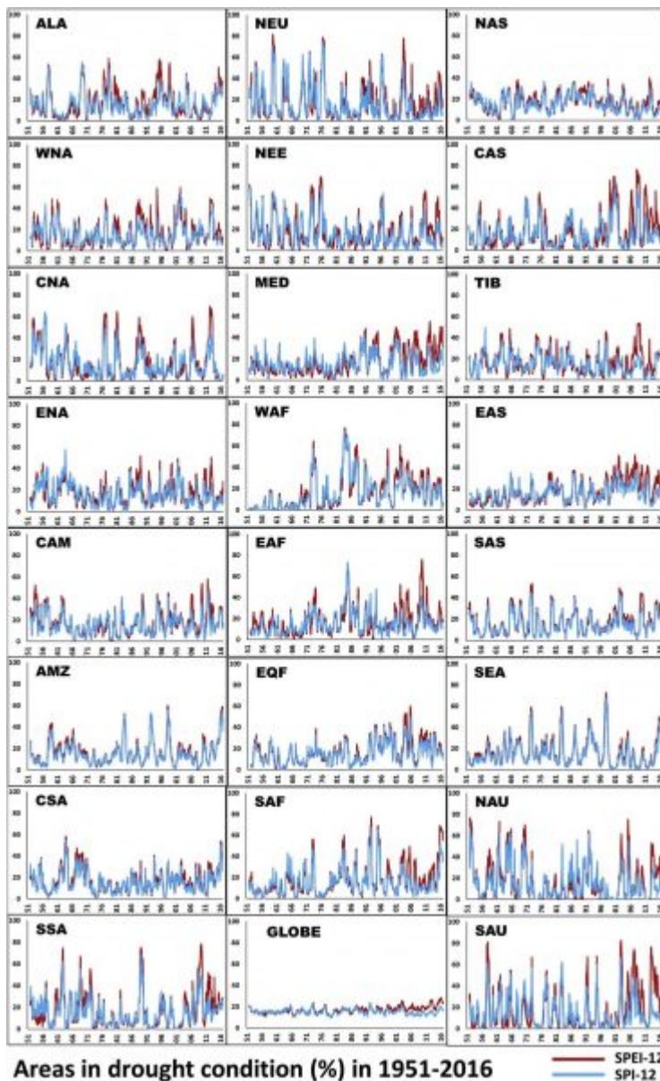
Bild 39 [8] Fig. 8. Percentage of areas in drought conditions from 1951 to 2016 according to the SPI-12 (blue) and to the SPEI-12 (red) for 23 macro-regions and at global level. For the list of the acronyms, see Table 1. (For interpretation of the references to colour in this figure legend, the reader is referred to the web version of this article.)
