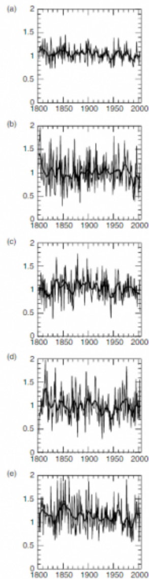
Figure 15. Average national precipitation series. (a) yearly series; (b) winter series; (c) spring series; (d) summer series; (e) autumn series. The series are displayed together with an 11-year window 3-year \sigma Gaussian low-pass filter
