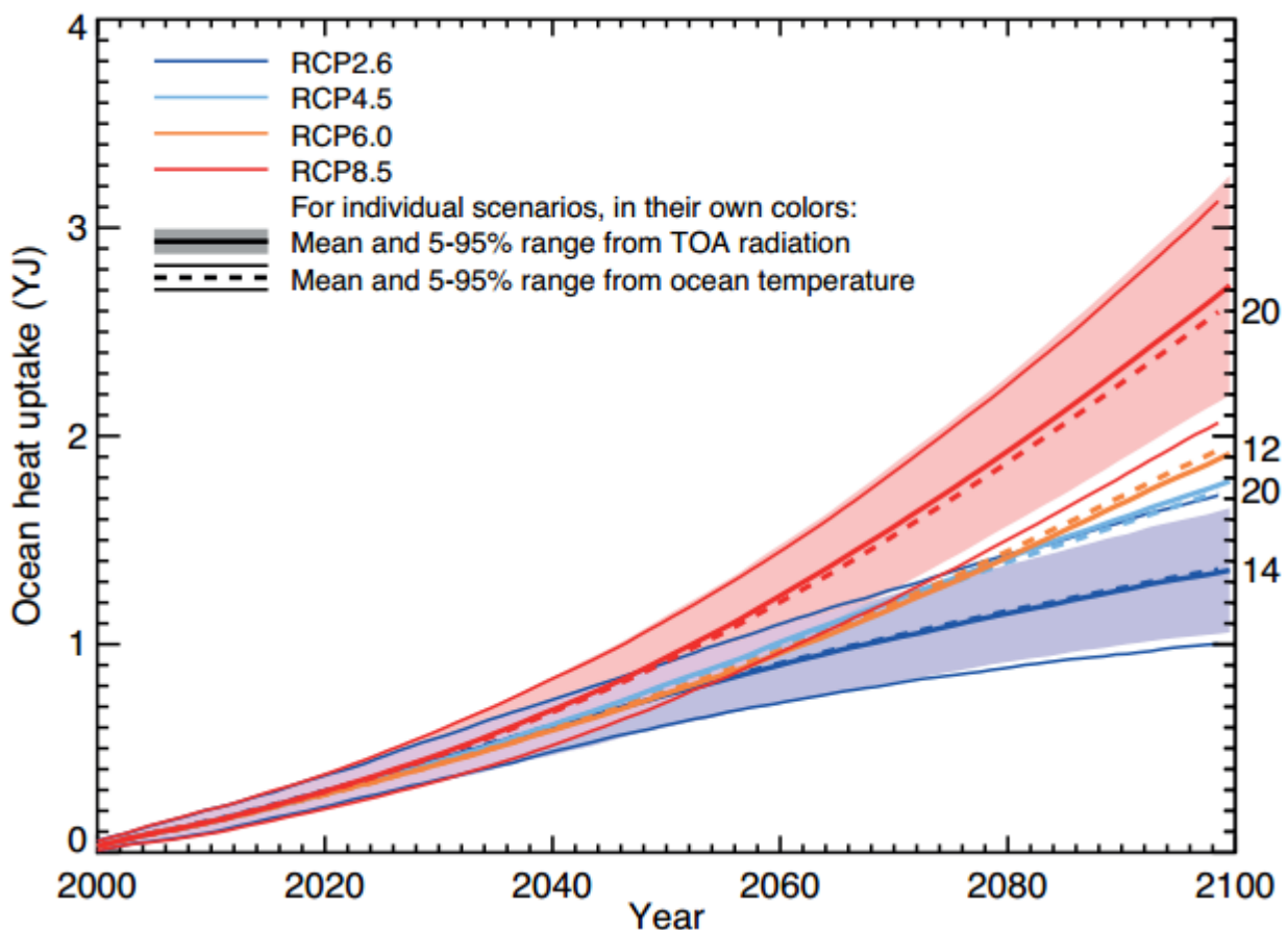
Bild 26 IPCC AR5 Figure 13.8 Heat uptake by the climate system during the 21st century relative to 1986–2005 projected by CMIP5 Atmosphere–Ocean General Circulation Models (AOGCMs) under RCP scenarios (1 YJ = 10 24 J).
