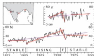
Figure 12. Tide gauge records from Mumbai (M) and Visakhapatnam (V) on each coast of India (location in the inserted map, where K stands for Korka and the present study area). The Mumbai (Bombay) record goes from 1878 to 1993. Unnikrishnan & Shankar [9] used a linear trend analysis (pink line) despite the fact that the records are composed of individual segments that must be treated individually (red lines). The individual segment analysis gives a totally different sea level story in 5 steps (division at base): stable, minor fall, general rise of 17 cm, rapid fall of 12 cm between 1955 and 1962, and full stability for the period after 1965. The last 5 steps are also recorded at Visakhapatnam (V).
