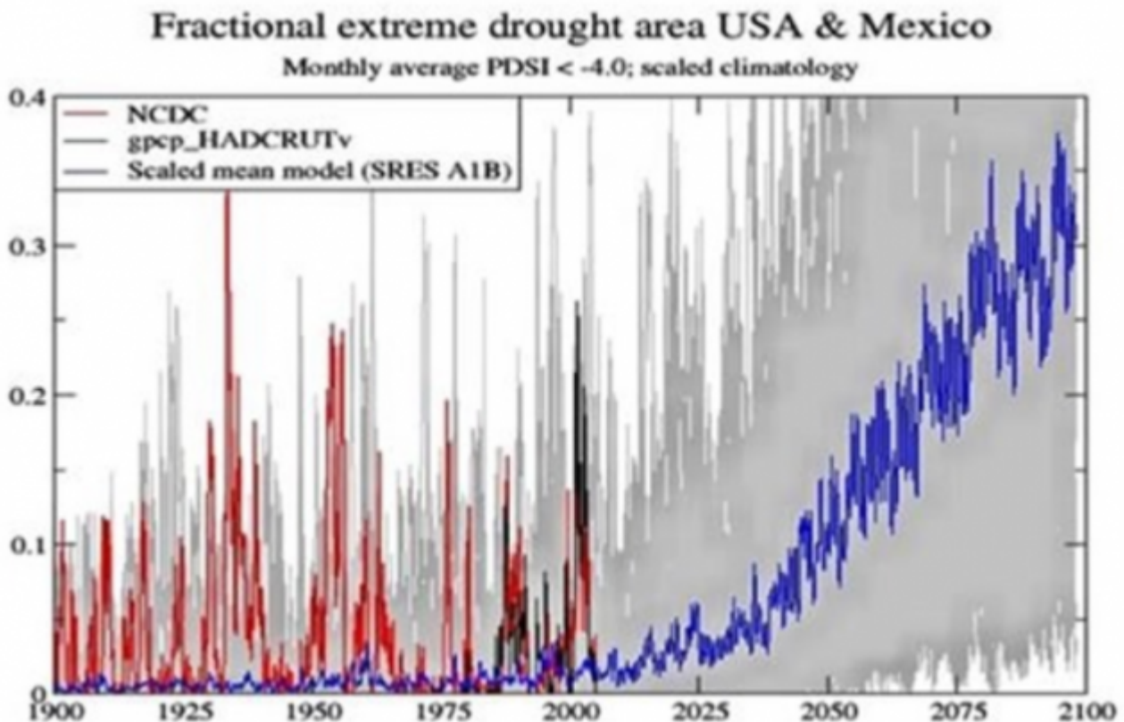
Bild 10 WUWT [10] Figure from Wehner et. al. (2011) Projections of Future Drought in the Continental United States and Mexico, Journal of Hydrometeorology
