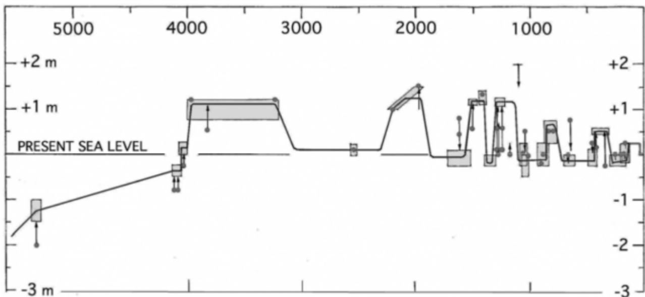
Bild 5 [16] Fig. 1. Sea level curve for the last 5000 years for the Maldives.
