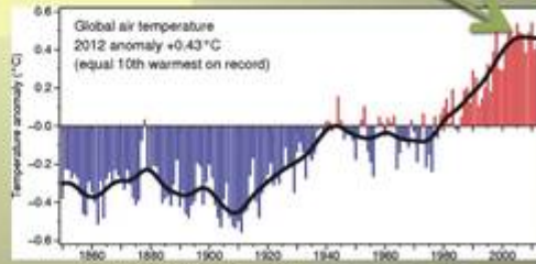
1: Global Temperature Record
