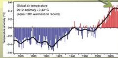
I: Global Temperature Record
