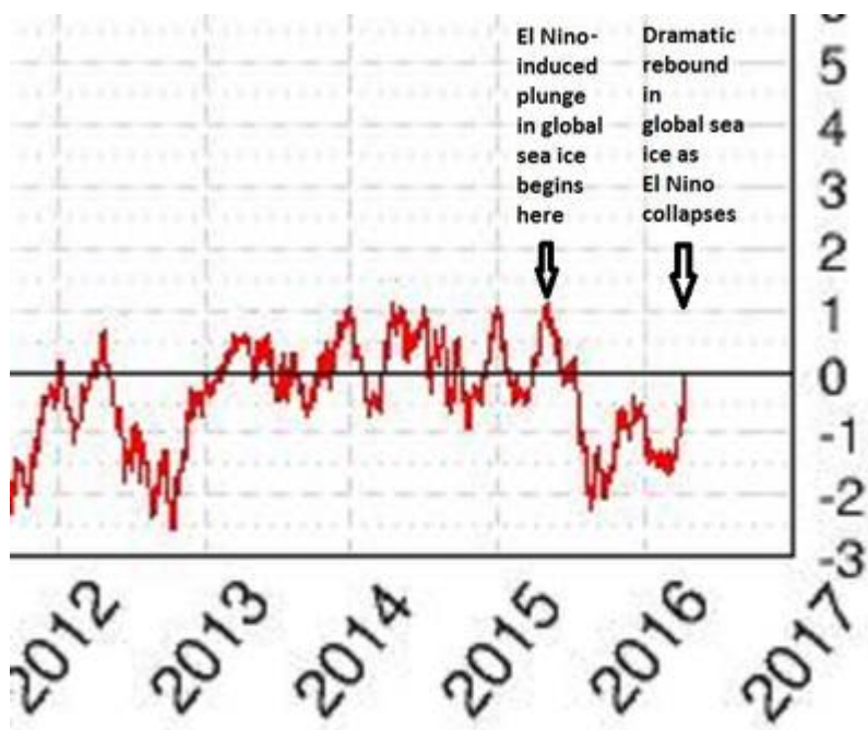
Daily global sea ice anomalies (in red) versus mean (1979-2008) [million sq km]
