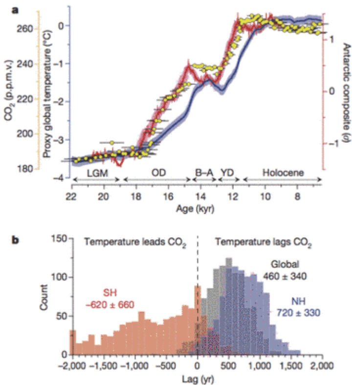
Figure 2 | CO 2 concentration and temperature. a. The global proxy temperature stack (blue) as deviations from the early Holocene (11.5–6.5 kyr ago) mean, an Antarctic ice-core composite temperature record 42 (red), and atmospheric CO 2 concentration (refs 12, 13; yellow dots). The Holocene, Younger Dryas (YD), Bølling-Allerød (B-A), Oldest Dryas (OD) and Last Glacial Maximum (LGM) intervals are indicated. Error bars, 1σ (Methods); p.p.m.v., parts per million by volume. b. The phasing of CO 2 concentration and temperature for the global (grey), Northern Hemisphere (NH; blue) and Southern Hemisphere (SH; red) proxy stacks based on lag correlations from 20–10 kyr ago in 1,000 Monte Carlo simulations (Methods). The mean and 1σ of the histograms are given. CO 2 concentration leads the global temperature stack in 90% of the simulations and lags it in 6%.
