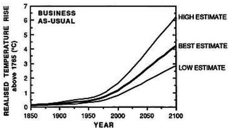
Figure 8: Simulation of the increase in global mean temperature from 1850-1990 due to observed increases in greenhouse gases, and prediction of the rise between 1990 and 2100 resulting from the Business-as-Usual emissions
