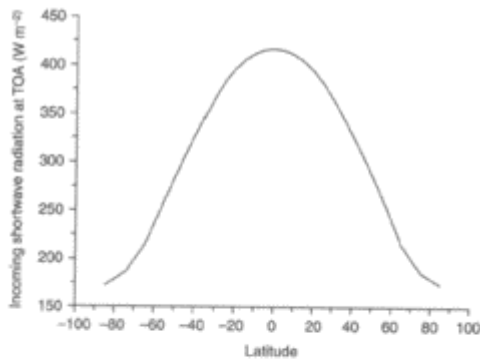
FIG. 5.17. Long-term (1984-1997) mean annual latitudinal variation of computed incoming shortwave radiation ( \text{W m}^{-2} ) at the top of the atmosphere. (Hatzianatassiou et al. 2004)
