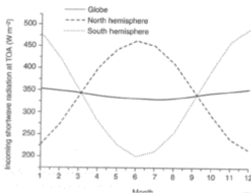
FIG. 5.18. Long-term (1984-1997) latitudinal average seasonal variation of incoming shortwave radiation ( \text{W m}^{-2} ) at the top of the atmosphere. (Hatzianatassiou et al. 2004)
