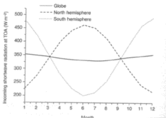
FIG. 5.18. Long-term (1984-1997) latitudinal average seasonal variation of incoming shortwave radiation ( \text{W m}^{-2} ) at the top of the atmosphere. (Hatzianatassiou et al. 2004)
