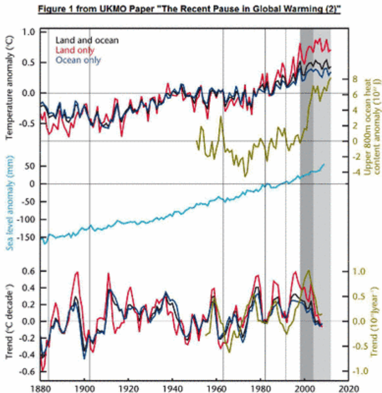
Figure 1: Observations of the recent pause in surface warming. Top panel shows time series of annual mean surface temperature anomalies (relative to 1961 to 1990) averaged over the whole globe (black, from HadCRUT4), land (red, from CRUTEM4) and ocean (blue, from HadSST3). The second panel shows the heat content of the upper 800m of the ocean (from Met Office analyses, anomalies relative to 1951 to 2006, updated from Smith and Murphy, 2007). The third panel shows annual globally averaged sea level from tide gauges (Church and White, 2011). The lower panel shows running nine-year trends in surface warming and upper ocean heat uptake. The recent slowdown in global warming is highlighted by the grey shading. This is split into onset (dark) and continuation (light) periods, where upper-ocean heat uptake increased during the onset, but was relatively flat during the continuation. Vertical lines indicate major volcanic eruptions.
