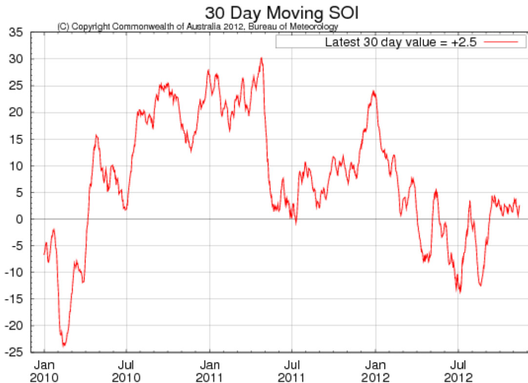
Abbildung 7 http://www.bom.gov.au/climate/enso/
