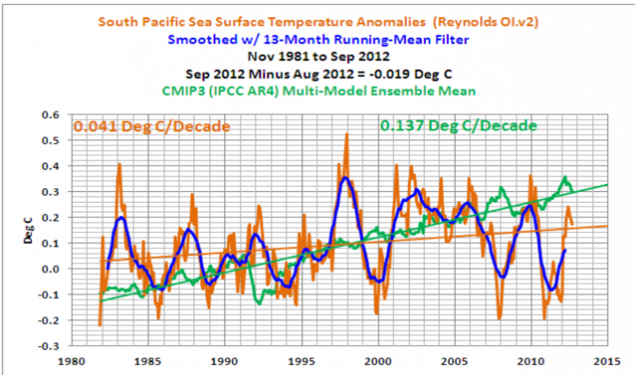
(9) South Pacific Sea Surface Temperature (SST) Anomalies (60S to 0, 120E to 70W)
