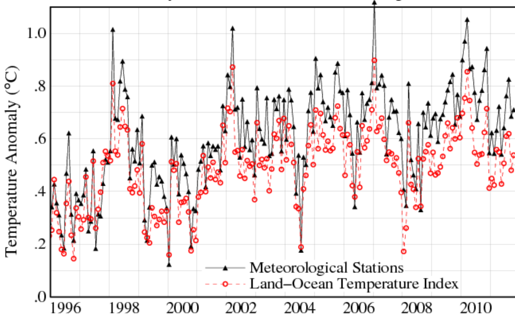
Monthly Mean Global Surface Temperature
