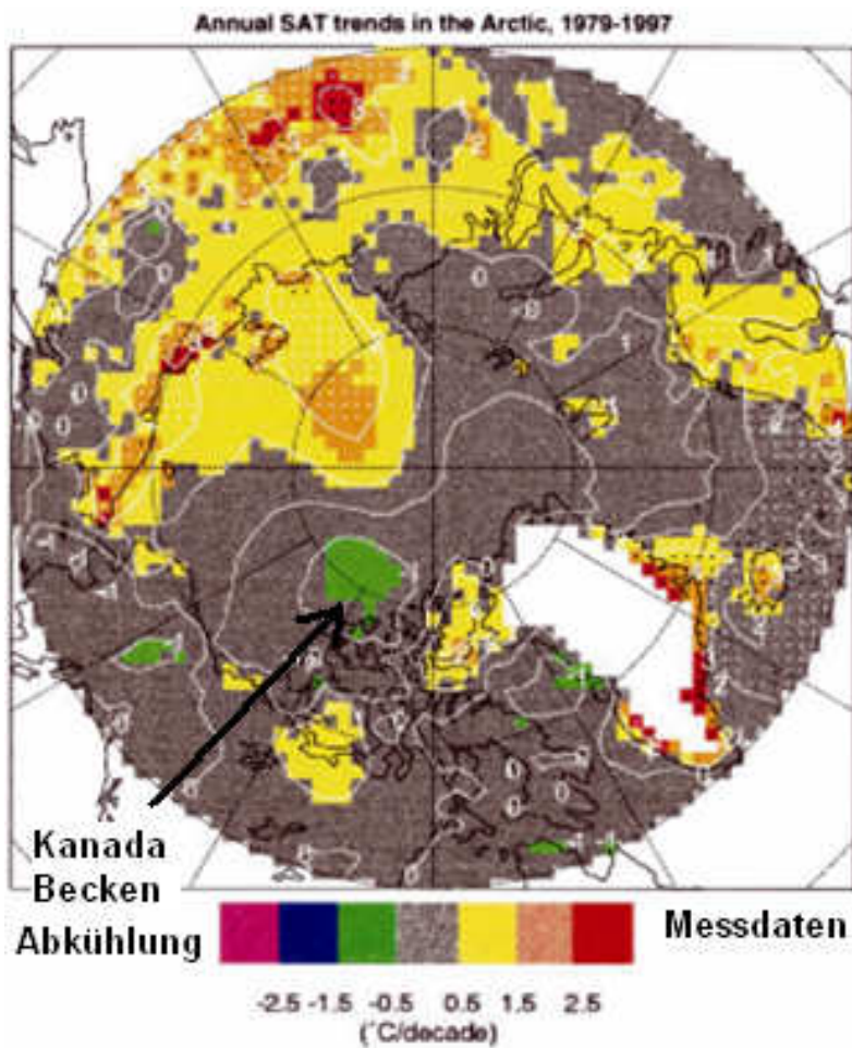
FIG. 8. Annual trends in SAT from IABP/POLES dataset for 1979-97
