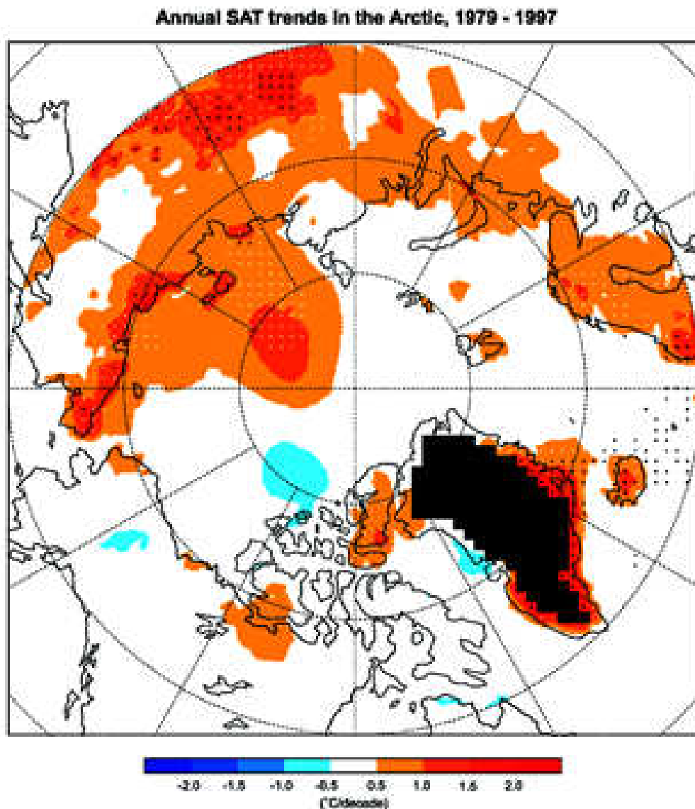
Figure 8. Annual SAT trends from IABP/POLES data set for 1979-1997.
