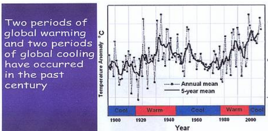
Figure 11. Temperature curve for the past century.
